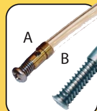
30 MIEHLE VERTICAL a- Air Release Valve. Used on feeder arm instead of #28 cap. Release a little air by turning screw. Excellent for cardboard and tissue. b- Cylinder Gripper, complete only. Fits all verticals.
